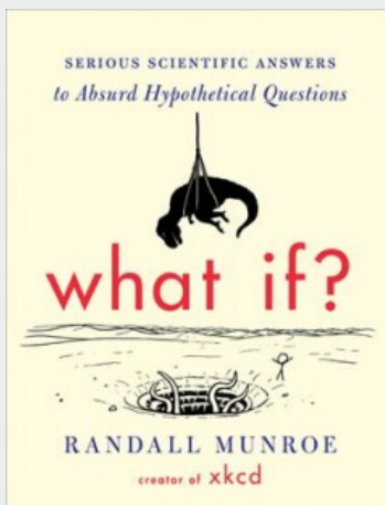
George's Pick
